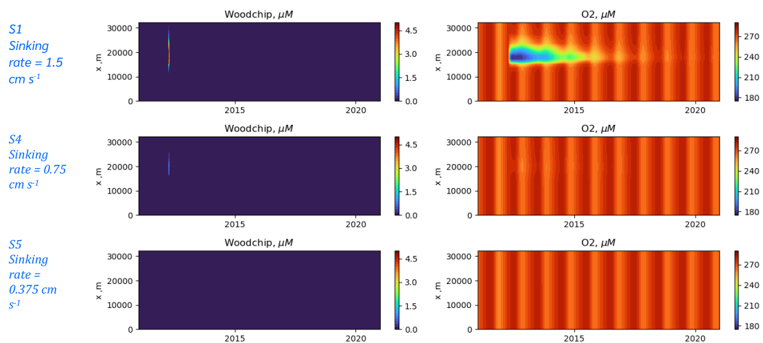
Figure 4.1. Interannual variability of woodchips ( \mu\text{M} ) and DO ( \mu\text{M} ) at the sediment surface with woodchip sinking rate 1.5 \text{ cm s}^{-1} (Scenario S1, top), 0.75 \text{ cm s}^{-1} (Scenario S4, middle), 0.375 \text{ cm s}^{-1} (Scenario S5, bottom).
