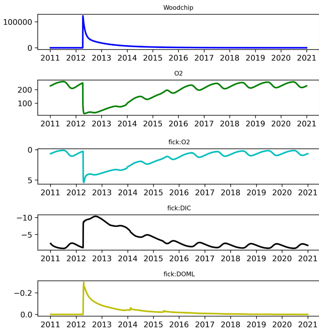
Figure 3.7. Interannual changes of bottom concentrations of woodchip ( \mu\text{M N} ), oxygen ( \mu\text{M} ) and bottom fluxes ( \text{mmol m}^{-2} \text{ day}^{-1} ) of oxygen (fick:o2), DIC (fick:DIC), and DOML (fick:DOML) (Scenario S1).
