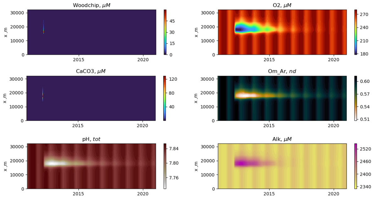
Figure 3.6. Interannual changes on the seafloor surface over a 10-year period; 1 year before woodchip deployment and 9 years after (95% woodchips + 5% \text{CaCO}_3 ; Scenario S1). Parameters include woodchips ( \mu\text{M N} ), oxygen ( \mu\text{M} ), \text{CaCO}_3 ( \mu\text{M} ), aragonite saturation, pH and alkalinity ( \mu\text{M} ). See Table 7.1 for full variable names.
