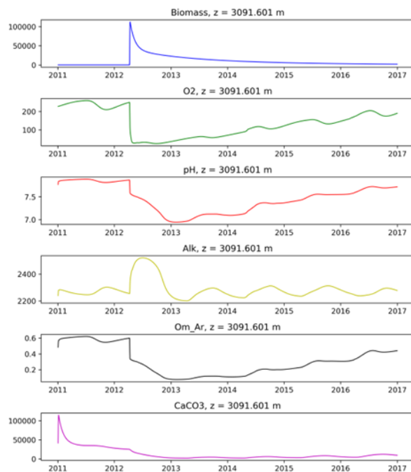
Figure 4.4. Interannual variability at the sediment surface of woodchips ( \mu\text{M N} ), oxygen ( \mu\text{M} ), pH, TA ( \mu\text{M} ), \Omega_{\text{ar}} , \text{CaCO}_3 ( \mu\text{M} ), in case of deployment of 100% of woodchips (left) and 95% of woodchips and 5% of \text{CaCO}_3 . The deployment occurred 01.04.2012 in model time.
