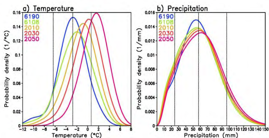
Figure 3.12. Probability distributions of (a) December mean temperature and (b) December precipitation sum in Helsinki, Finland. The blue and green lines represent the distributions derived from observations for 1961–1990 and 1961–2008, respectively, using Gaussian kernel smoothing. The yellow, red and purple lines give the model-based best estimates for the distributions around the years 2010, 2030 and 2050, respectively. The three vertical lines show the 10 th , 50 th and 90 th percentiles of the distributions for the reference period 1961–1990.
